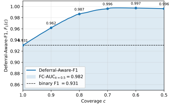
Fig. 8: Deferral-Aware-F1 curve of the logistic regression on the test set at threshold t^* = 0.56 with the FC-AUC shaded area.
