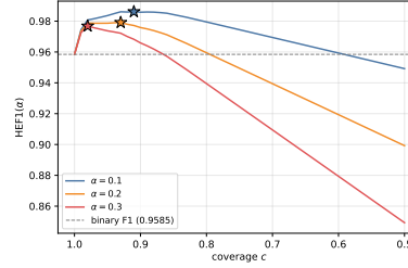
Fig. 10: \text{CAS}(\alpha) against coverage (two-sided); stars mark the per- \alpha optimum, dashed line the binary F1.
