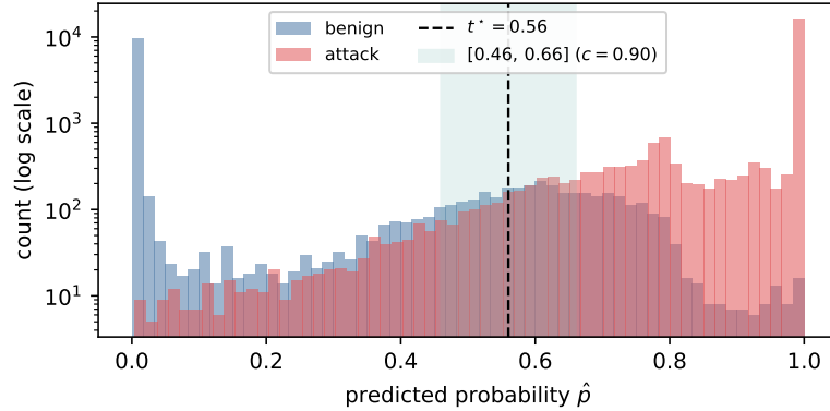
Fig 3: Distribution of predicted positive (‘attack’) probabilities \hat{p} . The tuned threshold is t^* = 0.56 with a confidence band is around it ( c = 0.90 ).
