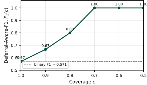
Fig. 2: Deferral-Aware-F1 curve on the 10-case worked example. The dashed line is the binary F1 (0.571).
