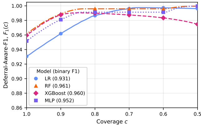
Fig. 4: Deferral-Aware-F1 as a function of coverage c on the full test set for the four classifiers. Coverage decreases (deferral increases) from left to right.
