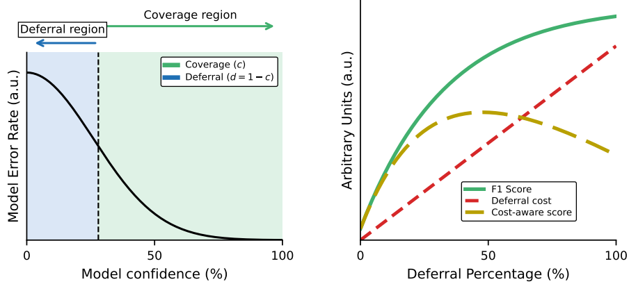
(a) Error rate by a model prediction's confidence: the 'coverage region' is where we want the model to decide, the 'deferral region' is the ideal set of decisions to defer to the human (i.e., 'low confidence').
