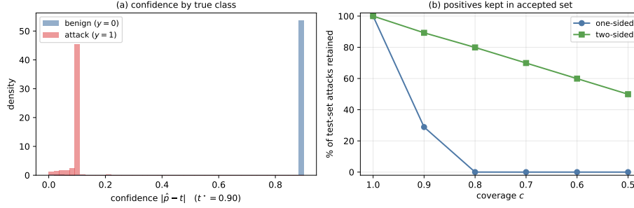
Fig. 9: (a) Confidence |\hat{p} - t| by true class: benign traffic is furthest from the threshold and is therefore ranked most confident. (b) Part of test-set attacks retained in the accepted subset as coverage falls.
