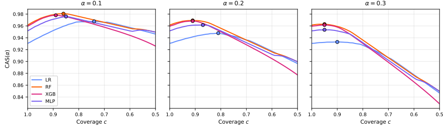
Fig. 6: CAS(\alpha) as a function of coverage c on the test set for the four classifiers. Each dot is a model optimum coverage c^* .
