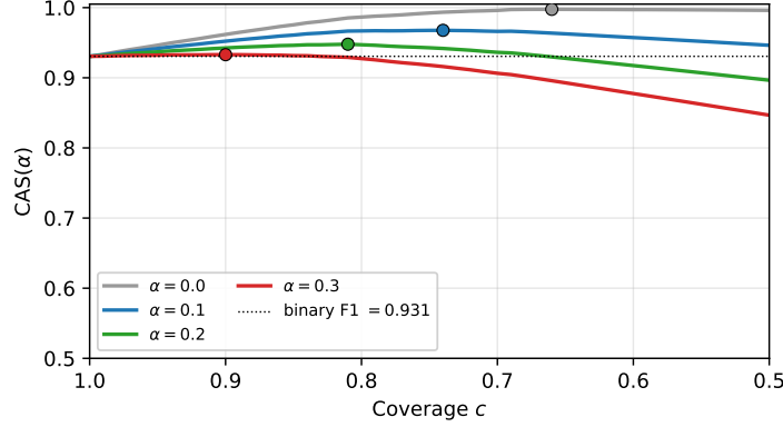
Fig. 5: CAS(\alpha, c) as a function of coverage c on the logistic regression. Each curve is one \alpha value and the point marks the maximum operating coverage c^* .
