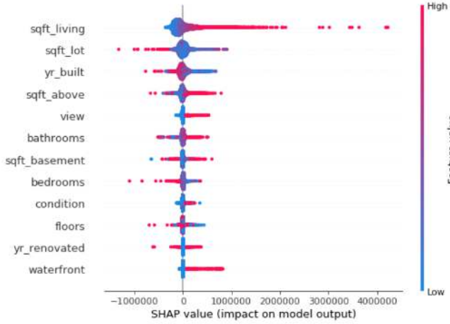
Fig. 3: Global Interpretation: Summary plot
