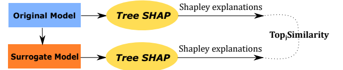
Fig. 5: Overview of the method calculating the Top_j Similarity metric
